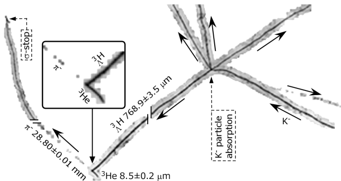
Figure 4. Firstly, detected scheme of production and decay of ^3_{\Lambda}\text{H} with overall-scanning method in Ref [7]. The original figure is presented in Ref. [21].
